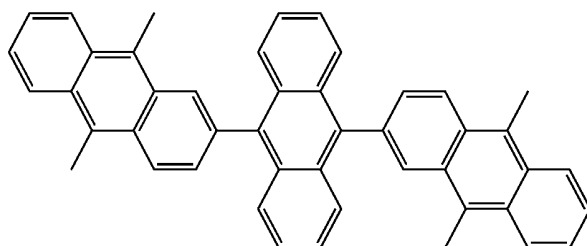
Structural formula A-26
