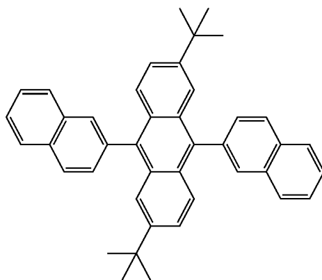
Structural formula A-32
