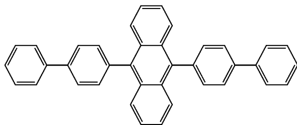
Structural formula A-4
