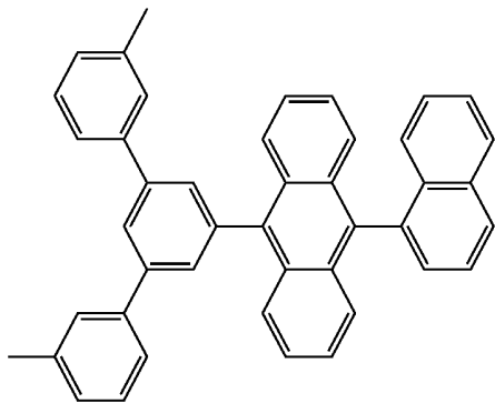
Structural formula A-48
