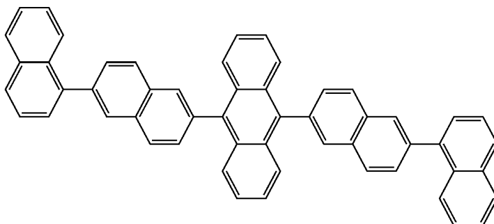
Structural formula A-24
