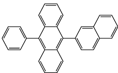
Structural formula A-41
